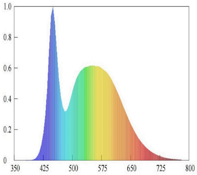
Spectral power distribution(6000K)
